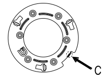
C: Bayonet of dome adaptor
