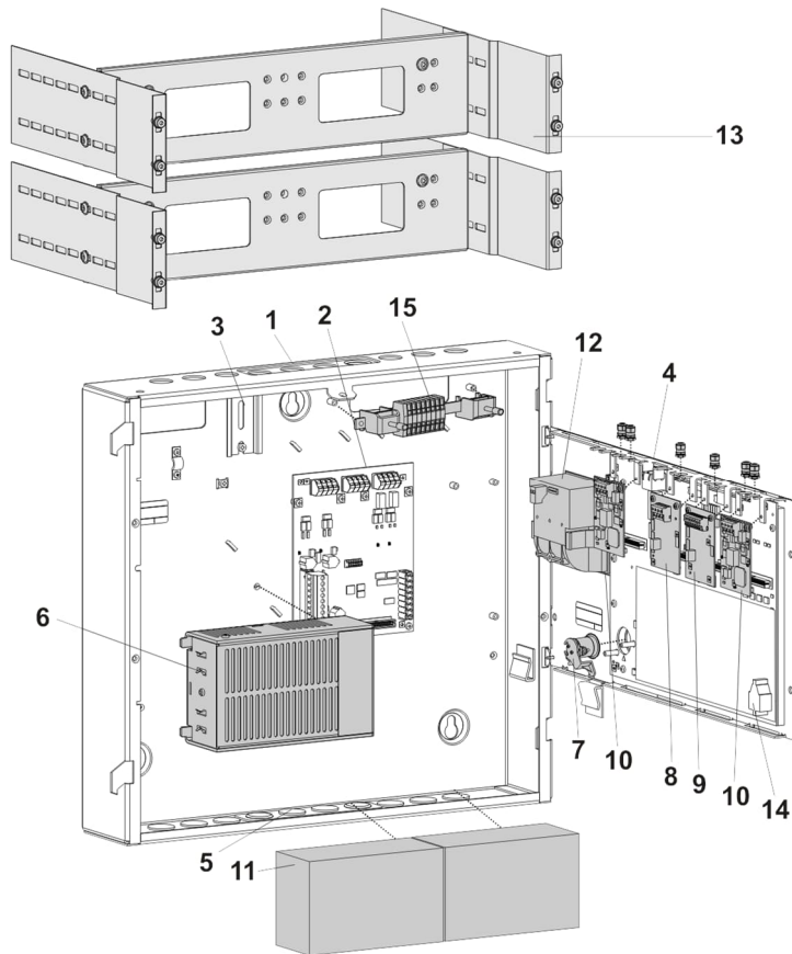
Fig. 5: Layout of FT724
