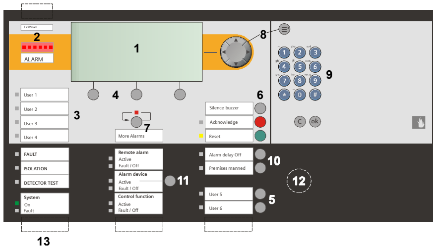
Fig. 4: Indication and operating elements
